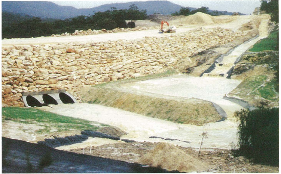
Above: Heavy rains during the construction period tested these erosion and sediment control works adjacent to Leask Creek.
