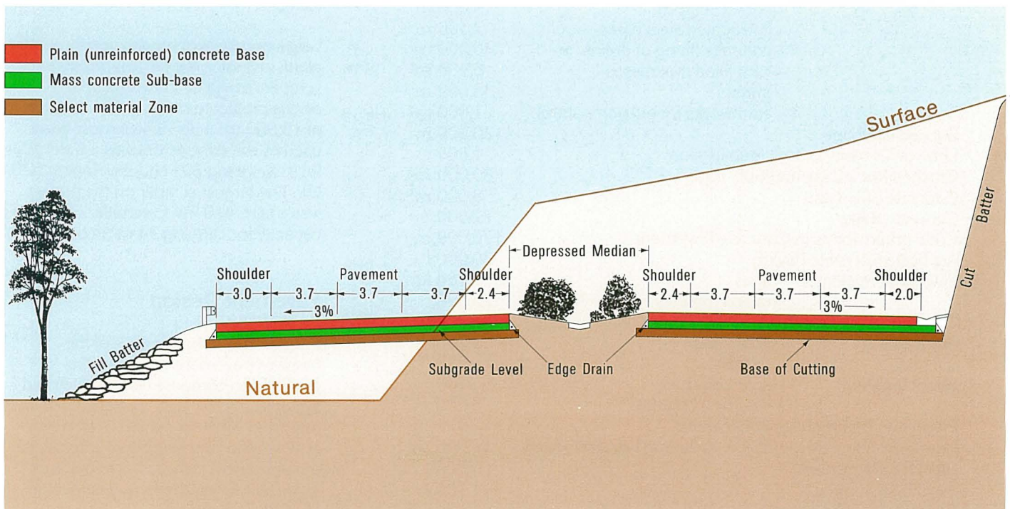
Freeway cross section on the approach to Mooney Mooney Creek Bridge
